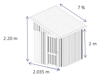
1 pente bac acier 7%
